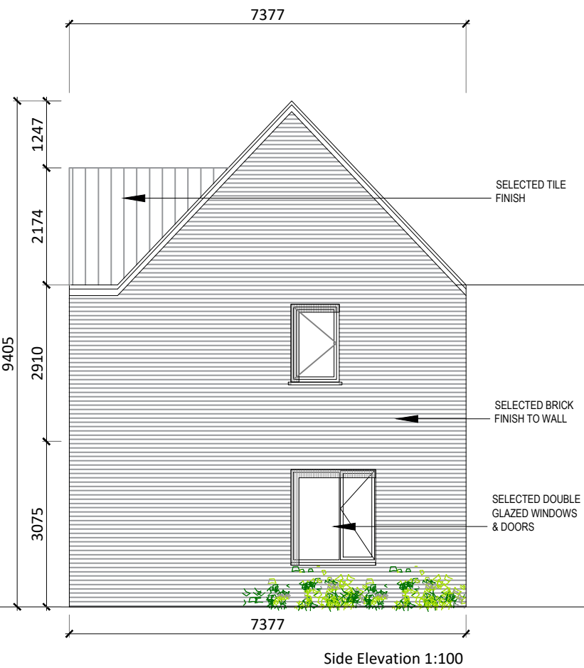
Side Elevation 1:100
