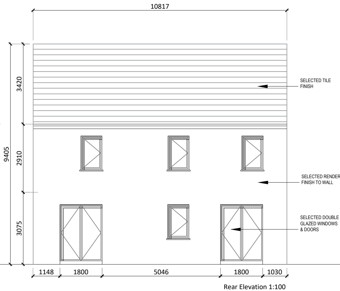
Rear Elevation 1:100
